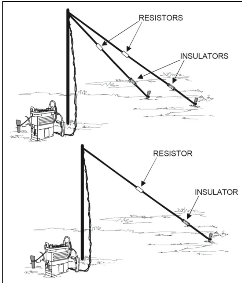
Figure 9-16. Sloping-V antenna
