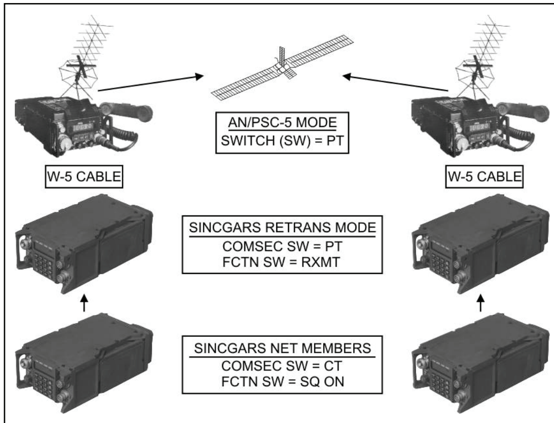
Figure 6-5. SINCARS range-extension with Spitfire
