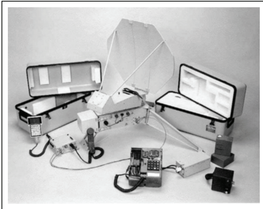
Figure 6-2. AN/PSN-11 SCAMP
