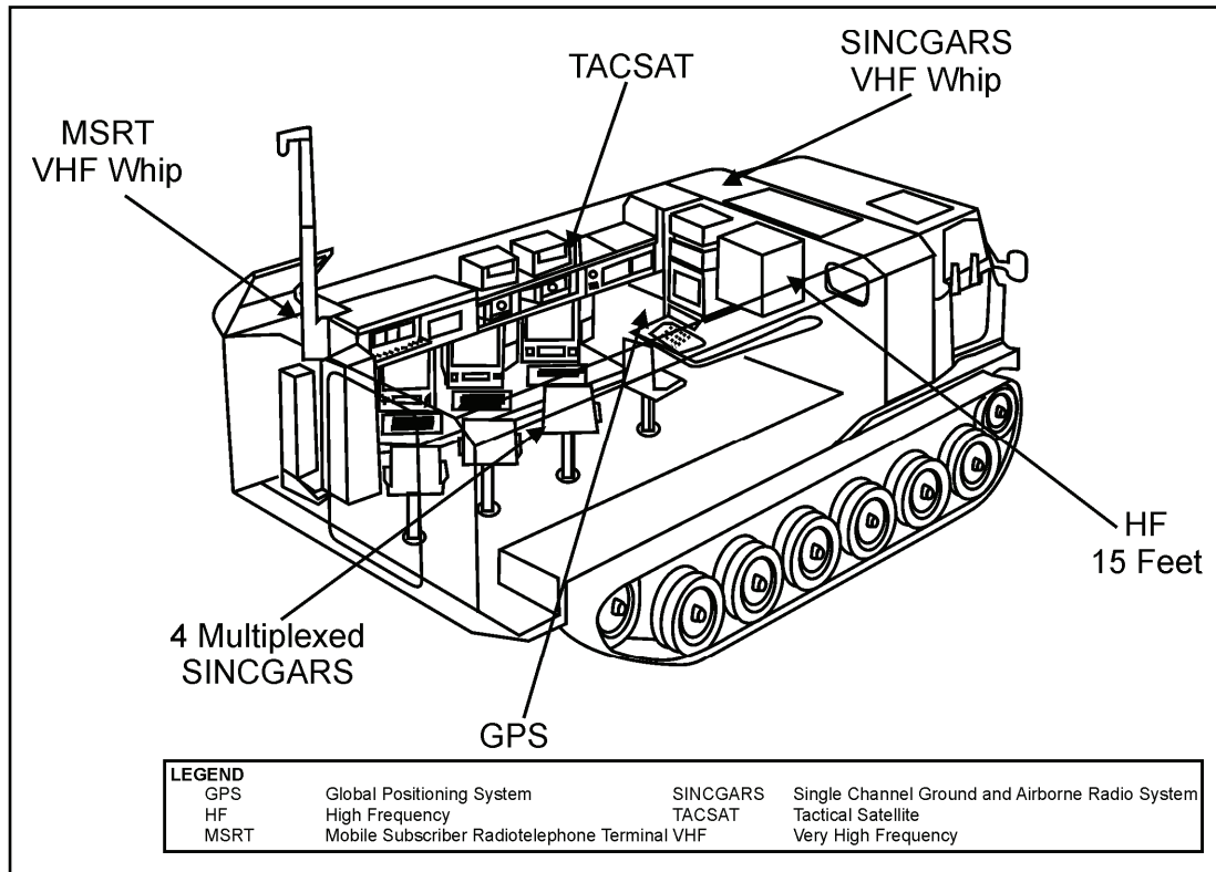
Figure H-1. Mobile command post antenna configuration
