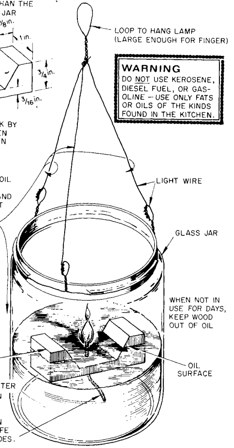
FLOATING WICK LAMP
