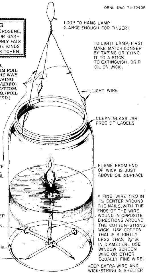
WIRE-STIFFENED-WICK LAMP
