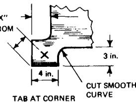
Fig. A. A dependable canopy to keep fallout and rain out of a vertical entry.
