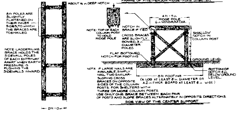
Fig. A.5. Aboveground, Ridgpole Shelter.
