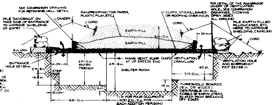
VIEW A-A, CROSS SECTION THROUGH LENGTH OF TRENCH SHELTER
