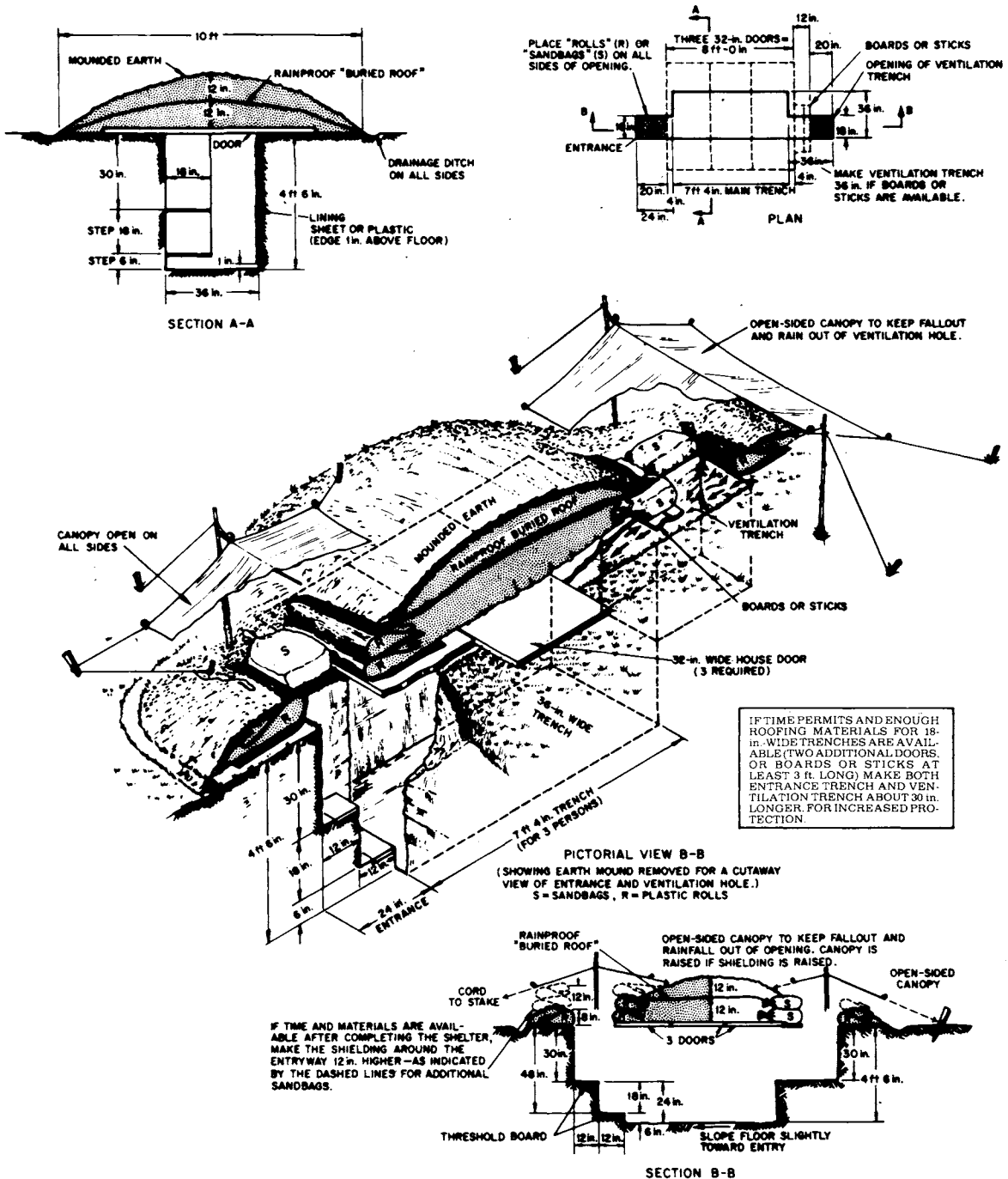
Fig. A.1. Door-Covered Trench Shelter. This file shared by Shane Connor of www.ki4u.com
