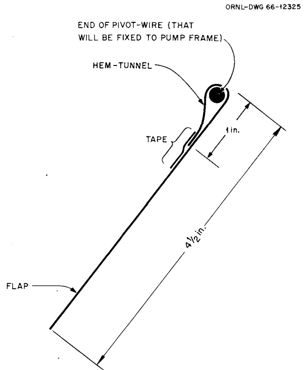
Fig. 7. End view.
