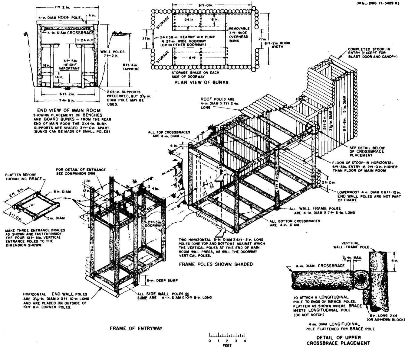
Fig. A.3.2. Pictorial View of Small-Pole Shelter. This file shared by Shane Connor of www.ki4u.com
