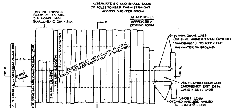
ROOF POLES - MINIMUM 7- ft LONG, 4- in. MINIMUM DIAMETER LAID ABOUT 2 ft. PAST EACH "D" OF SHELTER ROOM. PLAN VIEW OF TOP OF SHELTER SHOWING PLACEMENT OF POLES FOR ROOF (EARTH FILL NOT SHOWN)
